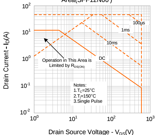
Figure 9-2. Max. Safe Operating Area(SFF12N60)
