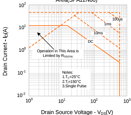
Figure 9-3. Max. Safe Operating Area(SFA12N60)
