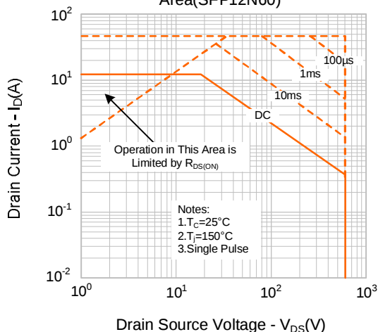
Figure 9-1. Max. Safe Operating Area(SFP12N60)
